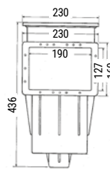
Skimmer dimension - standard track 3111
