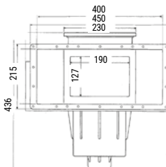
Skimmer dimension - wide track 3119
