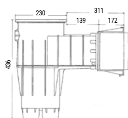
Skimmer dimension - wide track 3119
