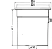
Water level regulator - 3150
