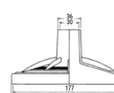
MasterFlo Skim-vac - 3190
