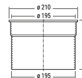
MasterFlo Extension collar - 3195
