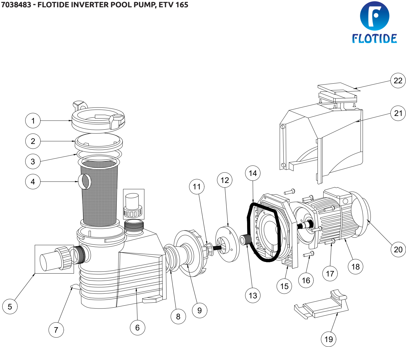
7038483 - FLOTIDE INVERTER POOL PUMP, ETV 165
