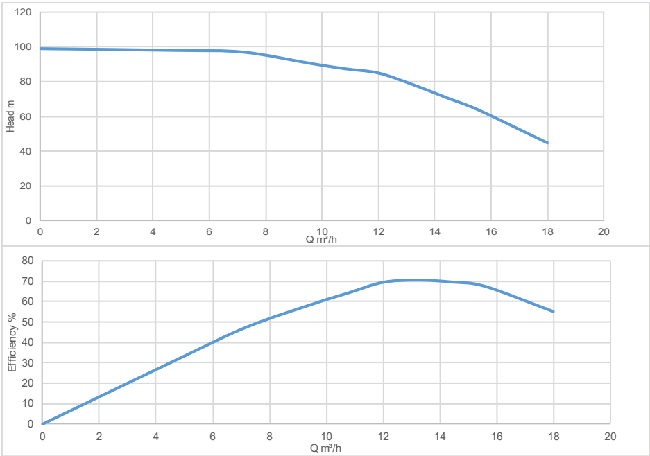
Performance Curve
