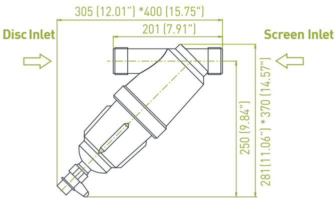
Dimentional Drawing
