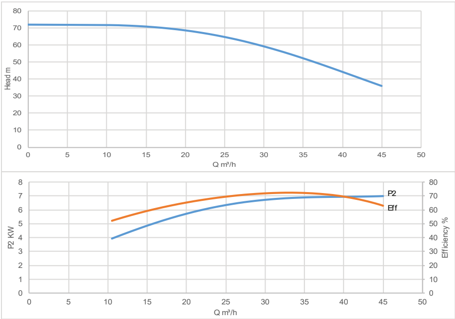
Performance Curve
