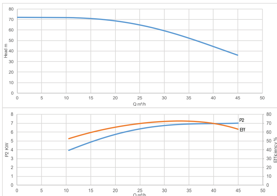
Performance Curve
