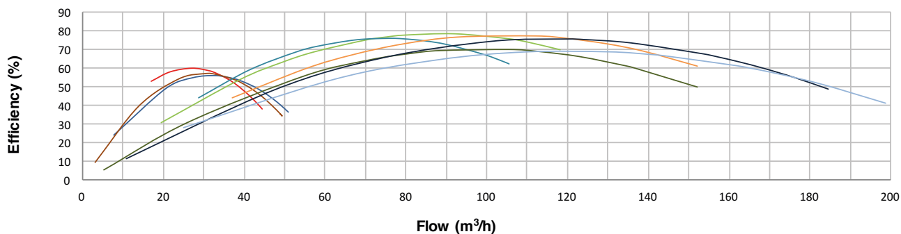
Hydraulic Performance
