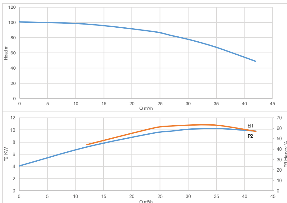
Performance Curve
